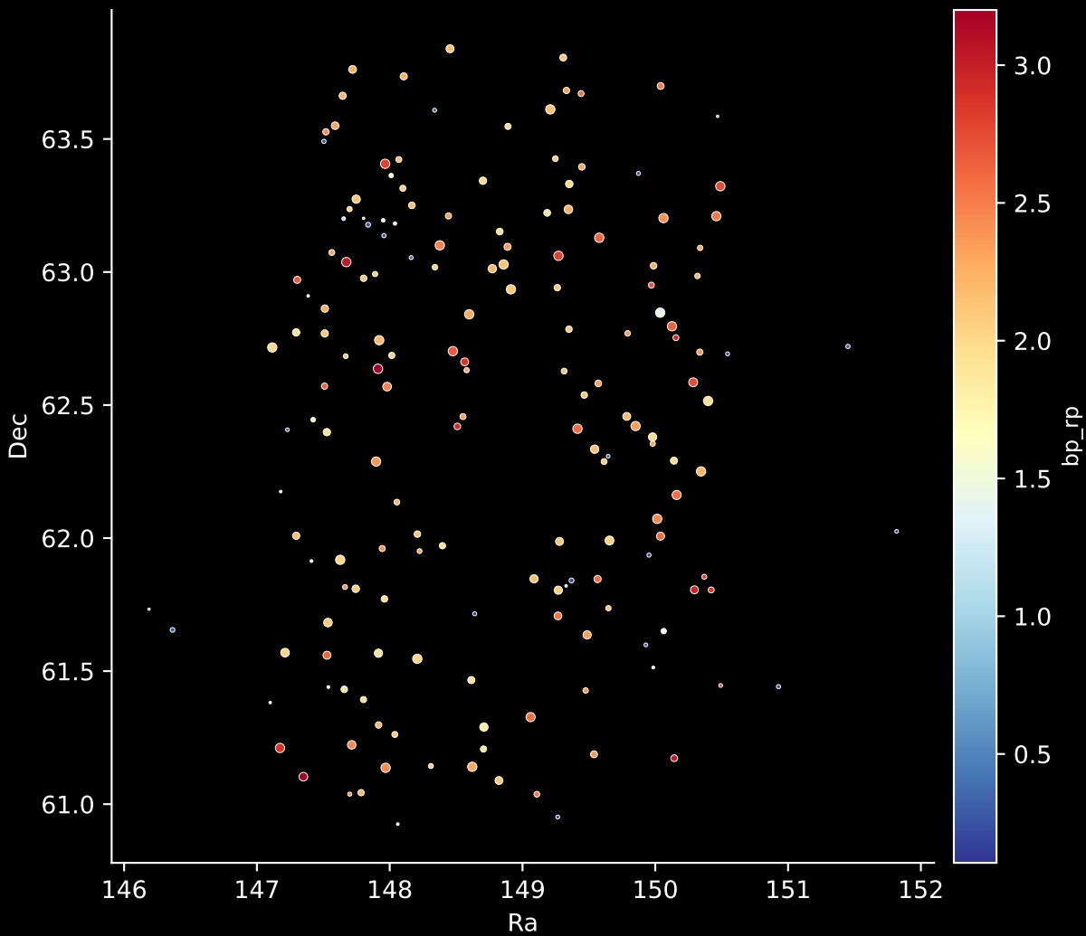
APOGEE DR17 Field: [139+04] Stars: 171
