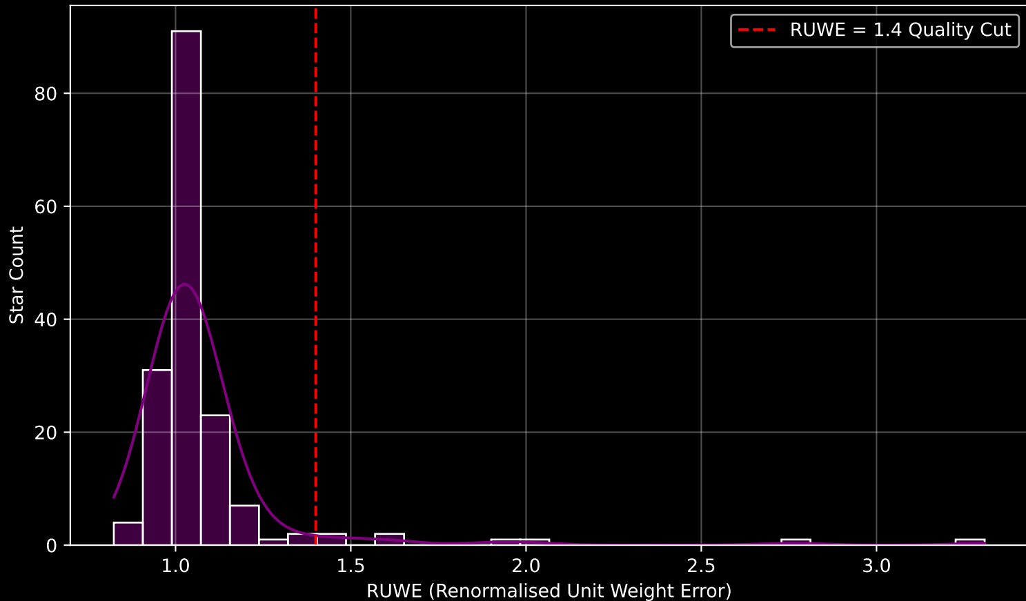
GAPOGEE DR17 Field [139+04] RUWE Distribution (n= 167)
