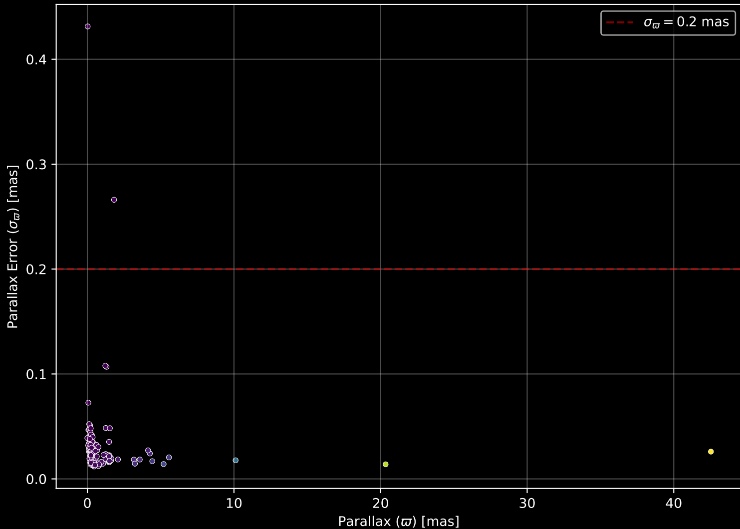
APOGEE DR17 Field: [139+04] Parallax Quality (n= 171)
