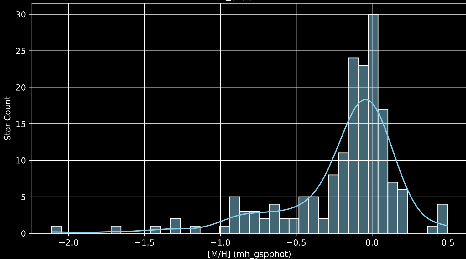
APOGEE DR17 Field: [139+04 [M/H] (mh_gspphot) (n= 171)
