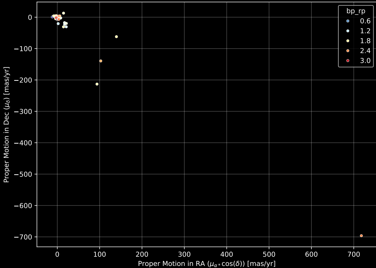
APOGEE DR17 Field: [139+04] Proper Motion Diagram (n= 171)
